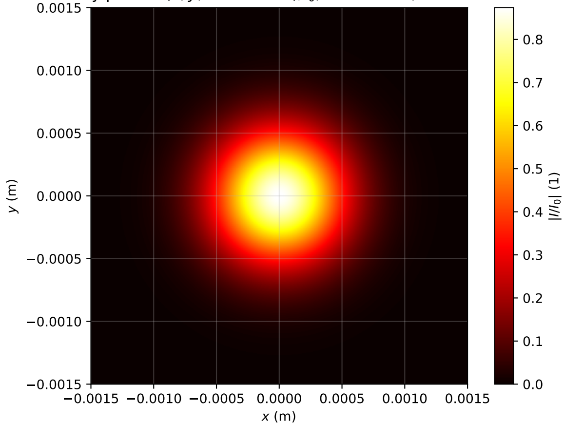
Intensity profile I(x, y, z = 0.876m)/I_0 , Pin=0.1Pcr, artificial time
